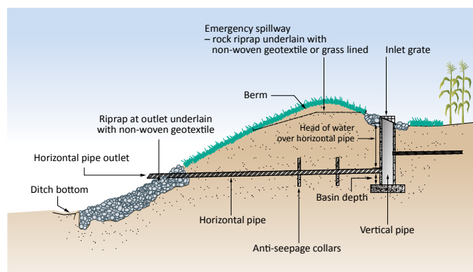
Figure B4-13. Drop inlet.
