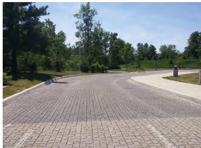
Figure B4-23. Permeable paving is used to increase the infiltration of water.
